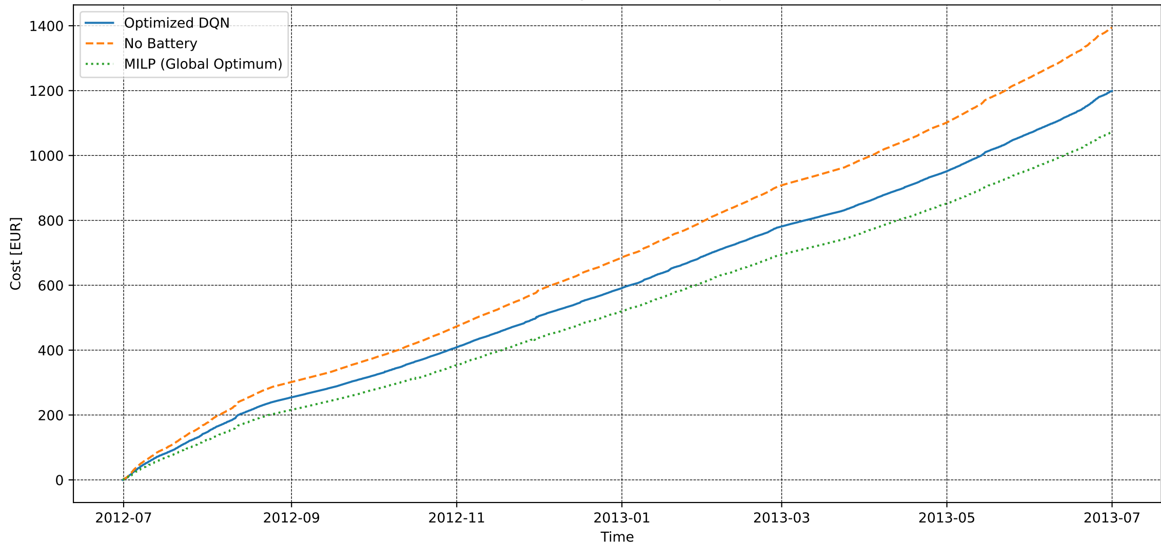
User 172 - Extended Convergence - Electricity Cost [DQN vs MILP]
